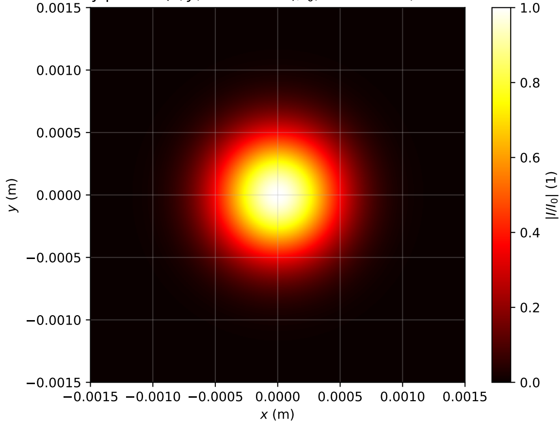
Intensity profile I(x, y, z = 0.000\text{m})/I_0 , Pin=0.5Pcr, artificial time
